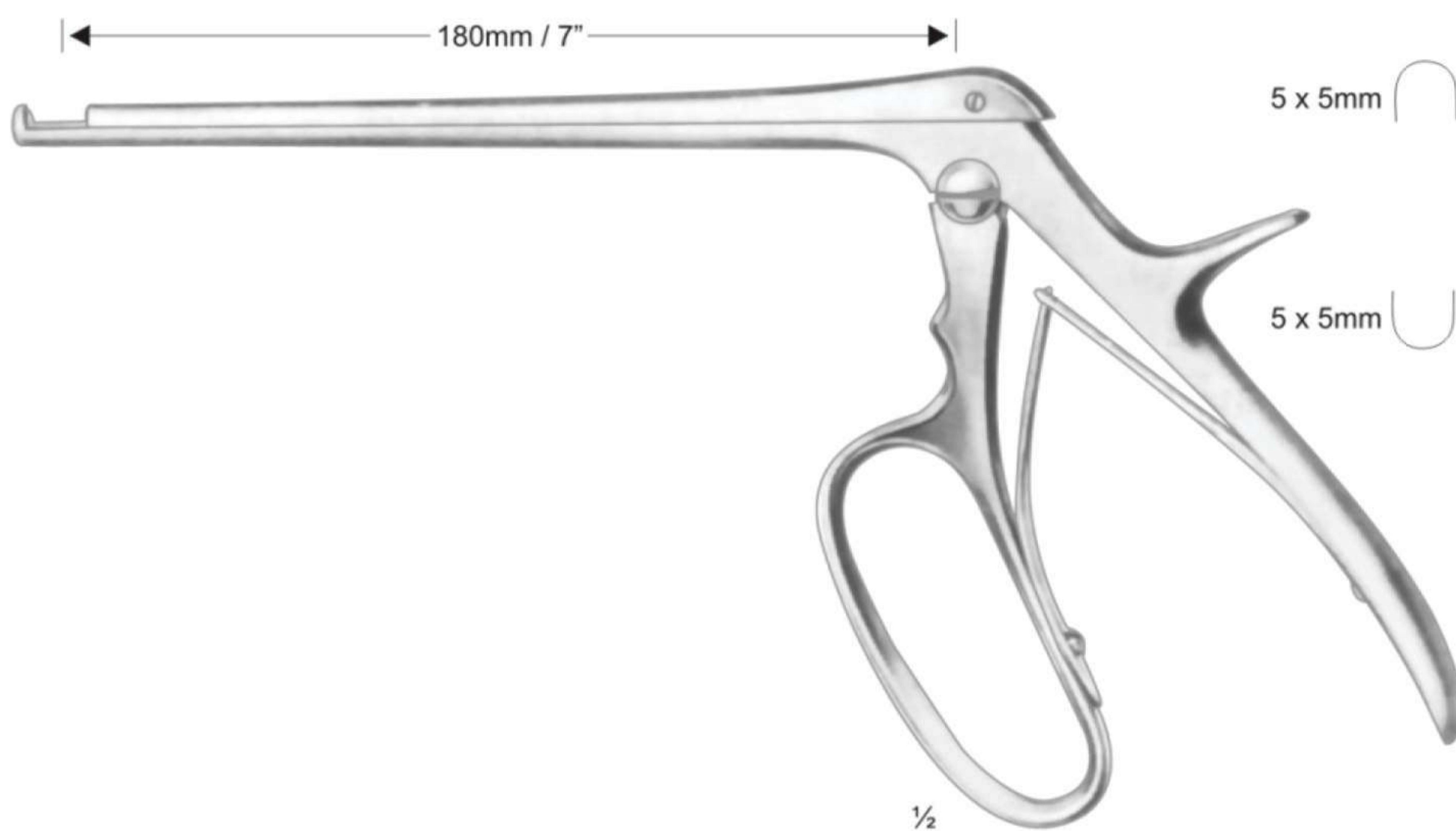
Ferris-Smith-Kerrison 18.0 cm / 7" shaft
